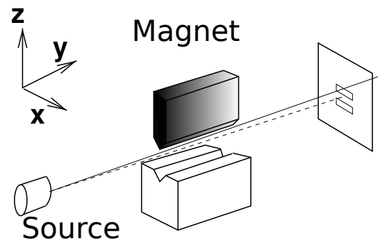
A schematic diagram of the Stern-Gerlach experiment.
